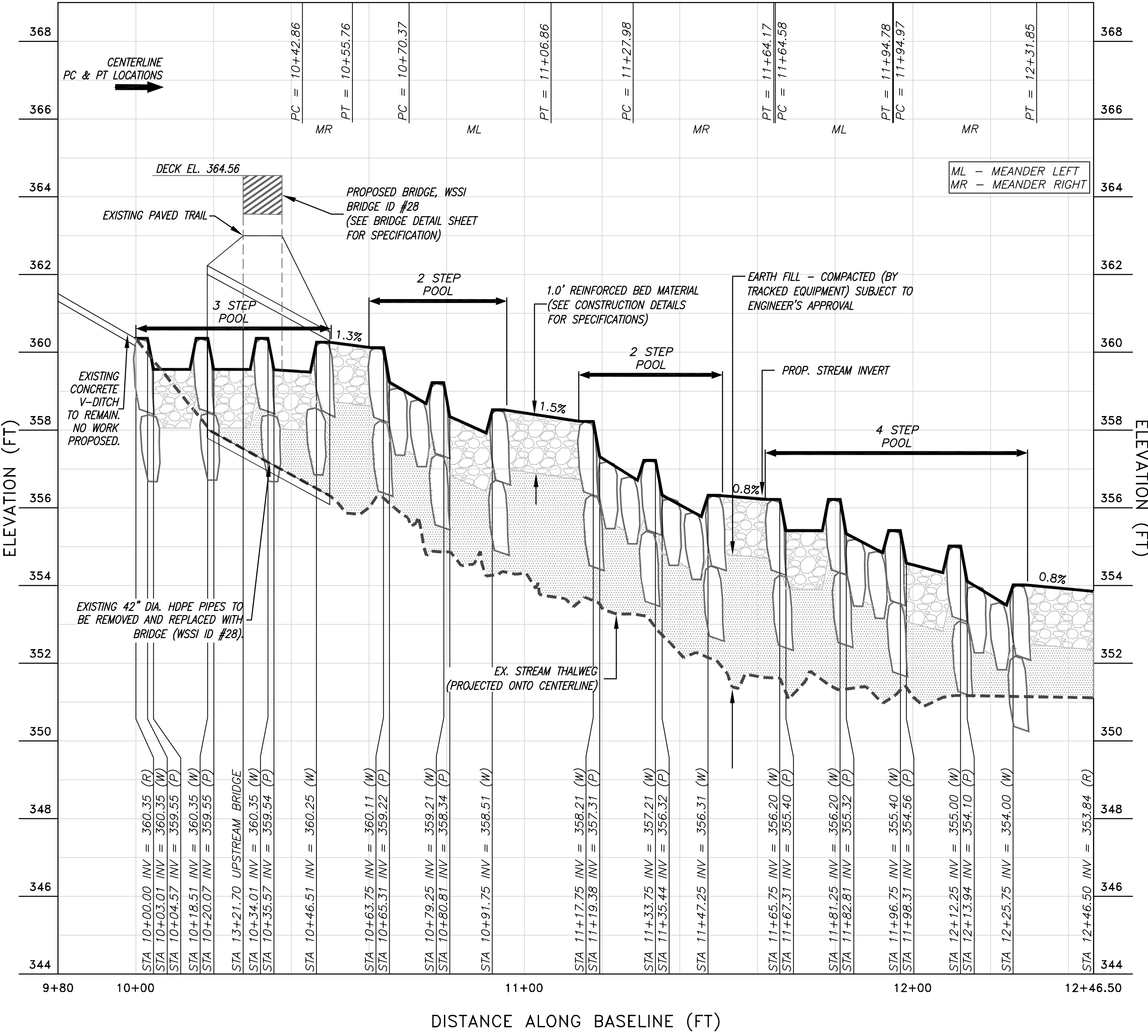
LONGITUDINAL PROFILE - TRIBUTARY 2 (STA 10+00 TO STA 12+47)
