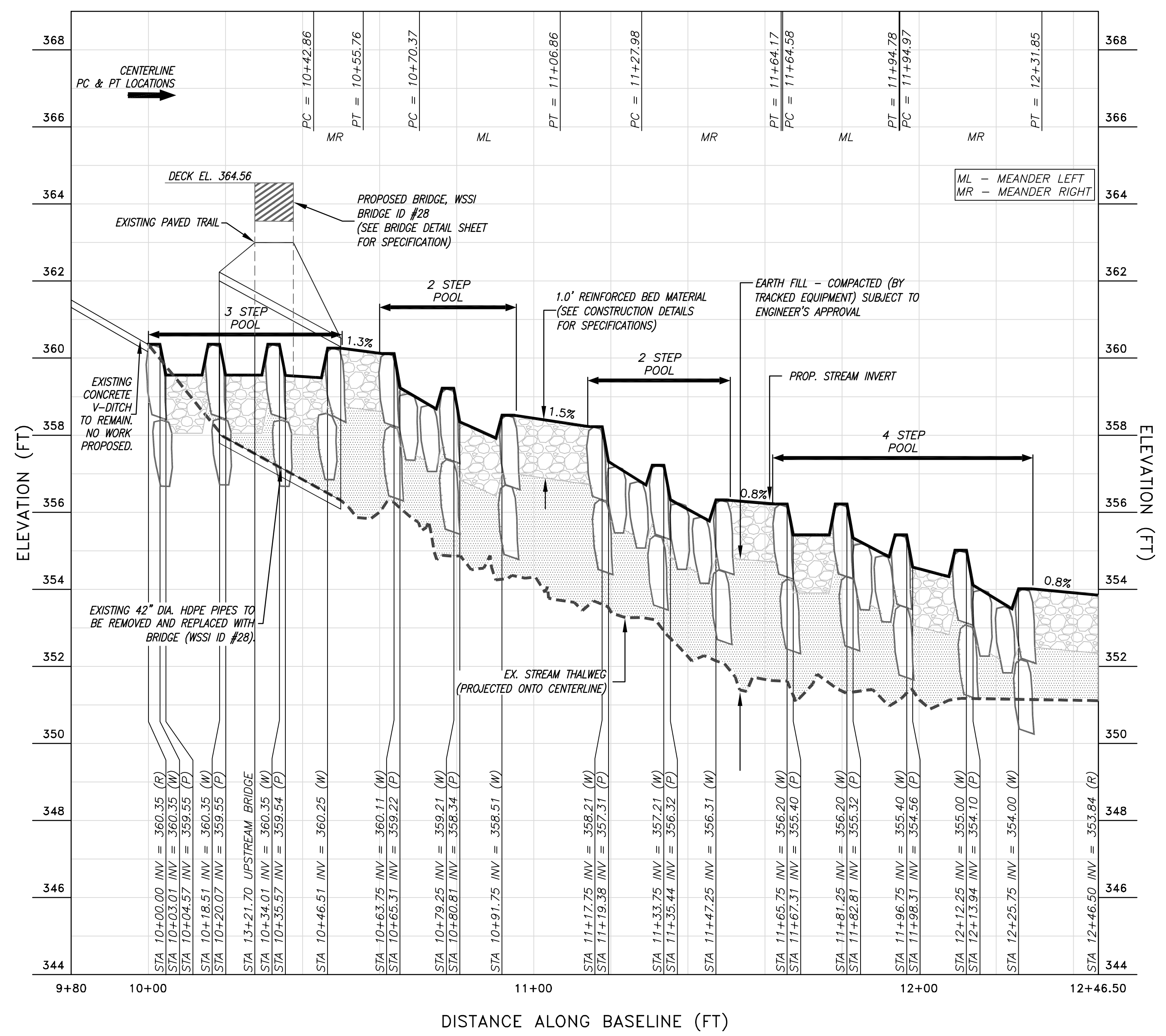
LONGITUDINAL PROFILE - TRIBUTARY 2 (STA 10+00 TO STA 12+47)
