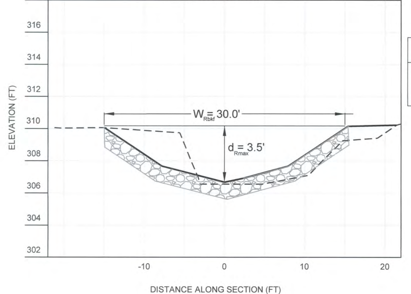
TYPICAL PROPOSED RIFFLE CROSS SECTION A-A' STATION 15+80
